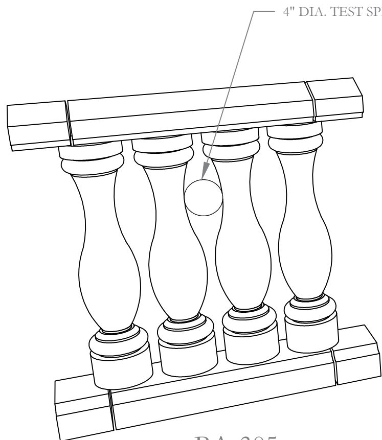
BA-305 Balustrade 7" O.C. per Code
