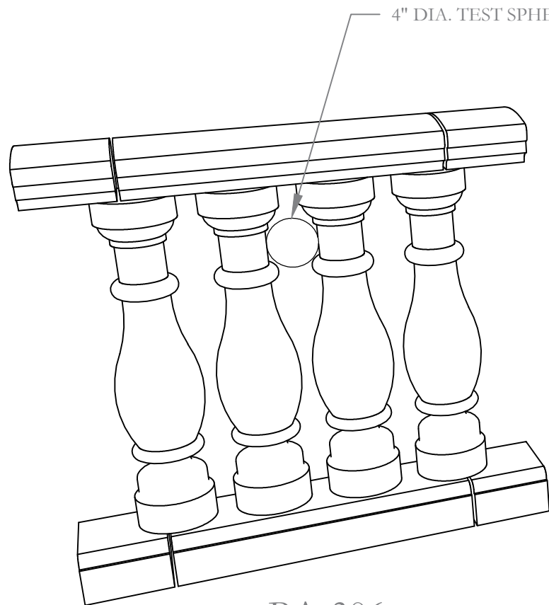
BA-306 Balustrade 7 1/2" O.C. per Code
