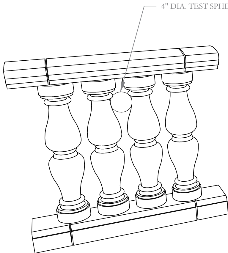
BA-307 Balustrade 7 7/16" O.C. per Code
