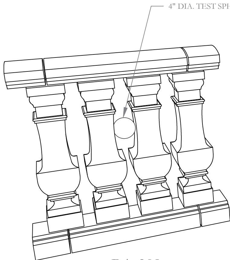
BA-309 Balustrade 8 1/4" O.C. per Code
