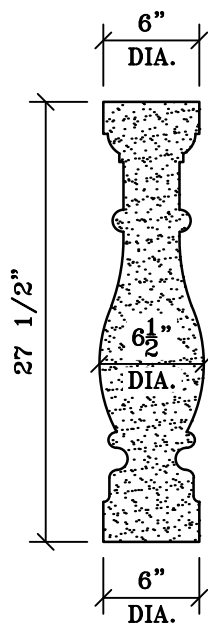
BA-306 Baluster Formerly BA301
