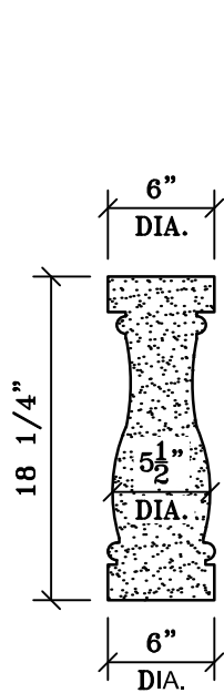
BA-301 Baluster Formerly BA308
