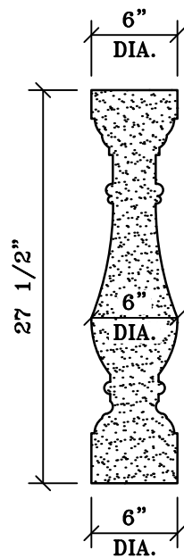
BA-302 Baluster Formerly BA302
