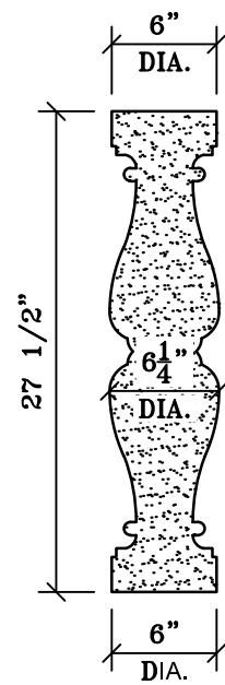
BA-307 Baluster Formerly BA305
