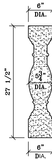
BA-304 Baluster Formerly BA303
