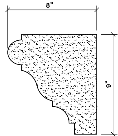
MO-922 Cornice Trim Formerly # CR105
