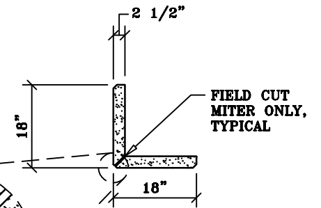
Field Mitered
