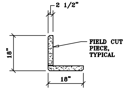
Butt Joint
