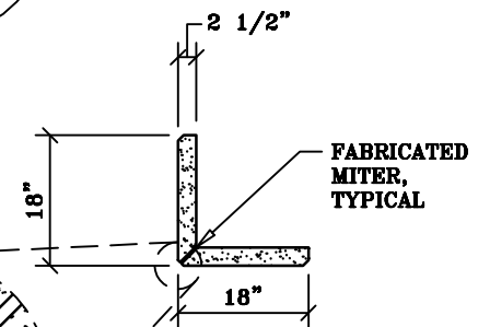
Quirk Mitered
