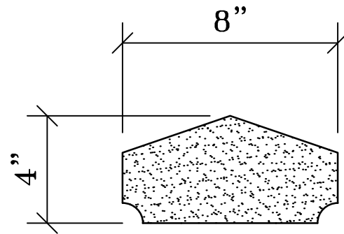
HR-322 Hand Rail Formerly HR322
