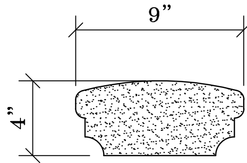
HR-323 Hand Rail Formerly HR321
