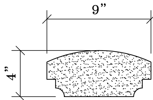
HR-324 Hand Rail Formerly HR323
