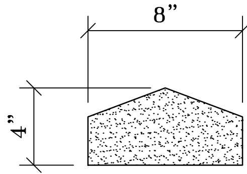
HR-321 Hand Rail Formerly HR320
