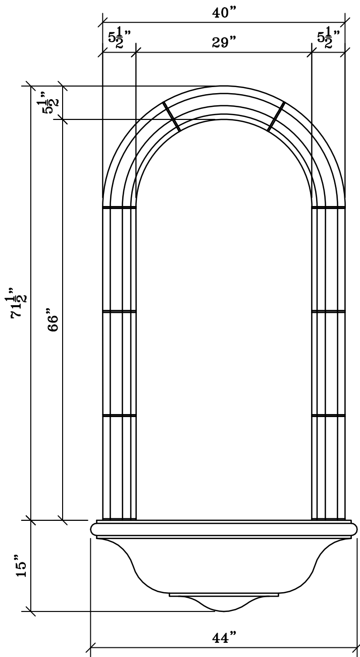
Front View NI-903
