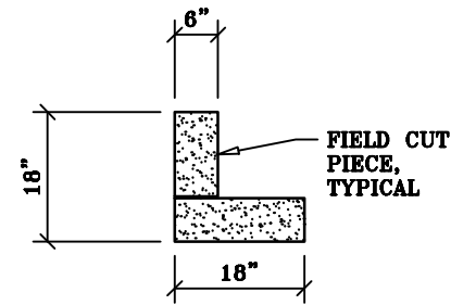
Butt Joint
