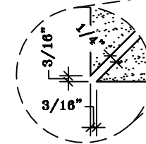
Field Mitered
