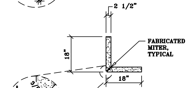
Quirk Mitered
