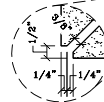
Quirk Mitered
