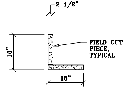
Butt Joint
